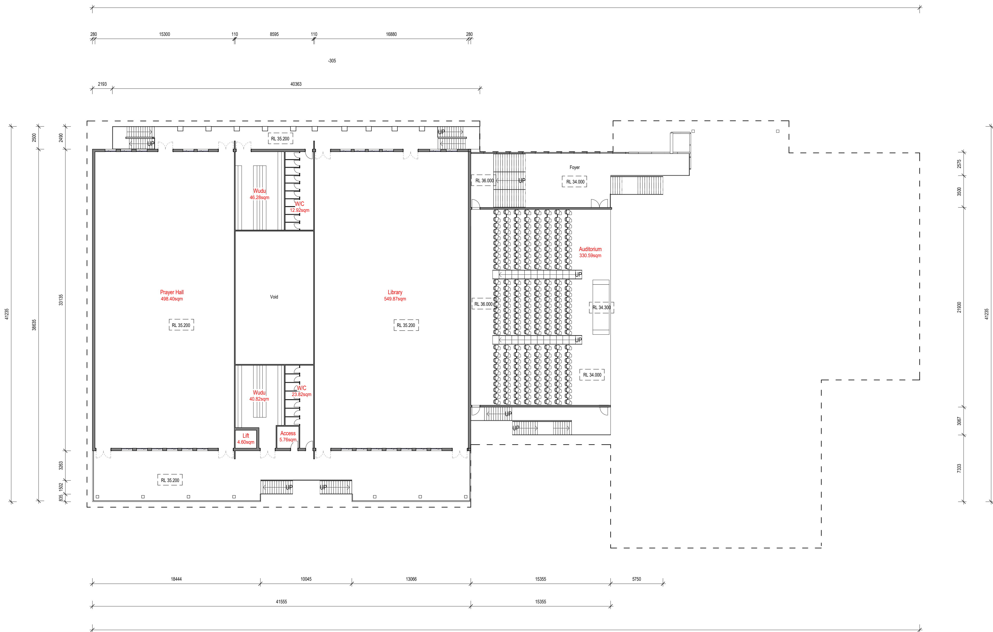
1 A- First Floor Plan 1 : 200
